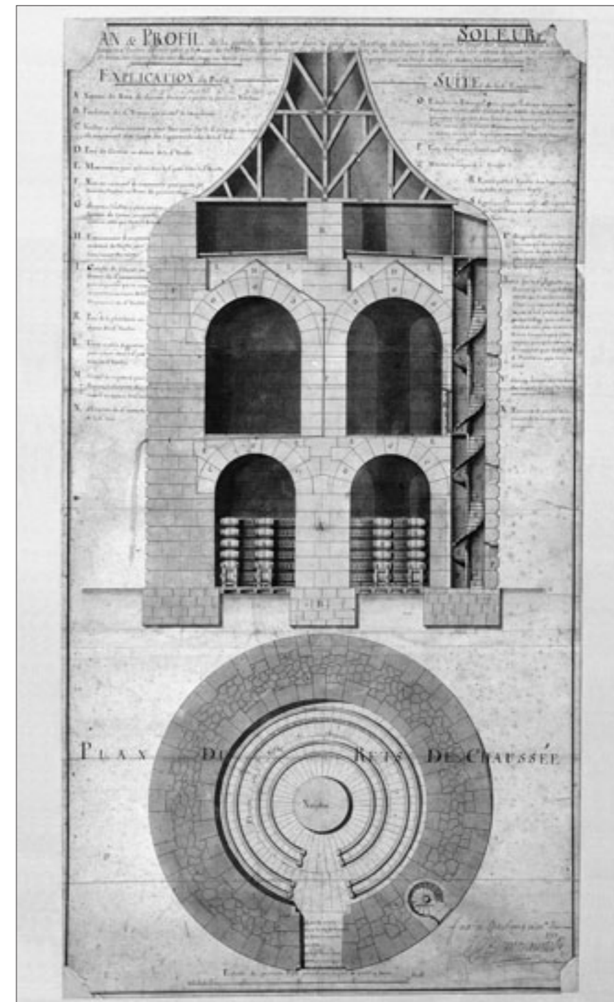
Abb. 3 Grundriss und Querschnitt durch den Riedholturm mit eingezeichnetem Projekt zum Einbau eines Pulvermagazins. Dated 18. Januar 1713, signed «Le. Demorainville», Strassburg. The tower served 1705 for a short time as a powder magazine, which in the immediate neighborhood, namely at the French ambassador's residence, highest inconvenience caused. In a letter he asked at that time the Solothurner Council with the request, the gunpowder elsewhere to store, as from one too great a danger. The project of 1713 was, although from the same ground, not carried out. (Source reference: RM 208/1705/560 vom 26. August 1705; Schanzratsmanual 1709–1713, Seite 120 links, Eintrag vom 21. Dezember 1712.)
