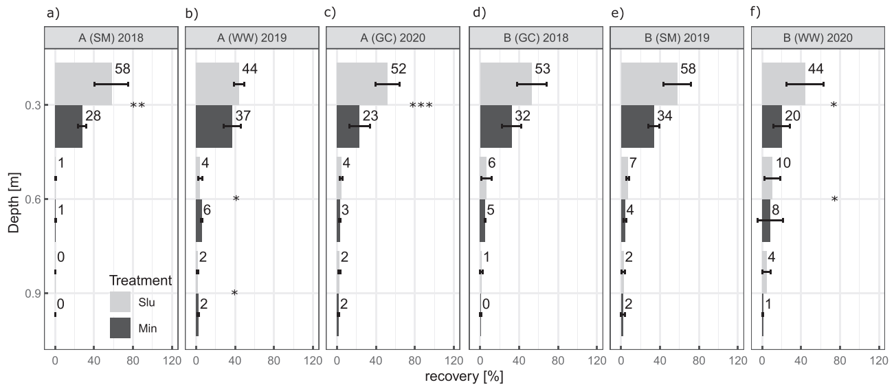
Fig. 4. ^{15}\text{N} recovery in soil relative to originally applied fertiliser for Field A (a–c) and for Field B (d–f). Samples in 2018 and 2019 were taken at the end of the vegetation period in mid-October, while sampling in 2020 took place upon harvest of the grass-clover in April (Field A) or upon harvest of winter wheat in July (Field B). SM = silage maize, WW = winter wheat, GC = grass-clover mean \pm standard deviation, n = 4 , with * ( p < 0.05 ), ** ( p < 0.01 ), and *** ( p < 0.001 ).
